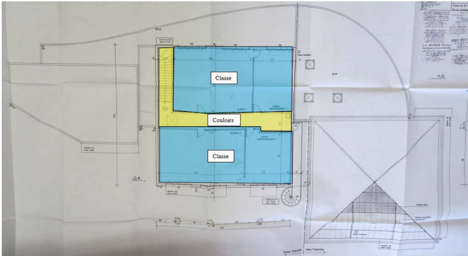
Plan R+1 Extension
